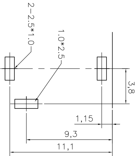
P.C.B. HOLE LAYOUT (BOTTOM VIEW)
